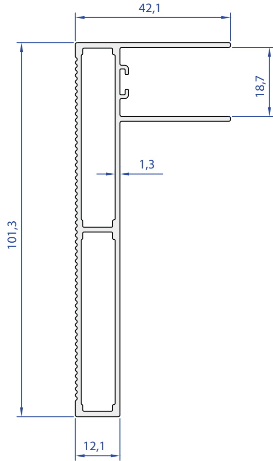
75354-00 1,093 Kg/m
