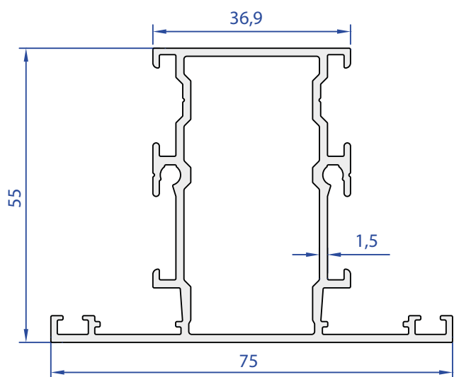
81007-16 1,138 kg/m
