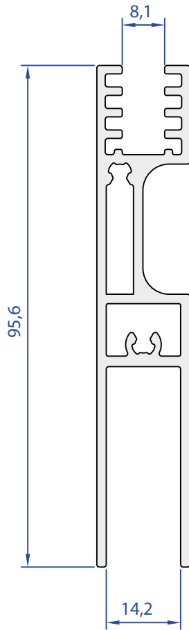
75422-00 1,310 Kg/m
