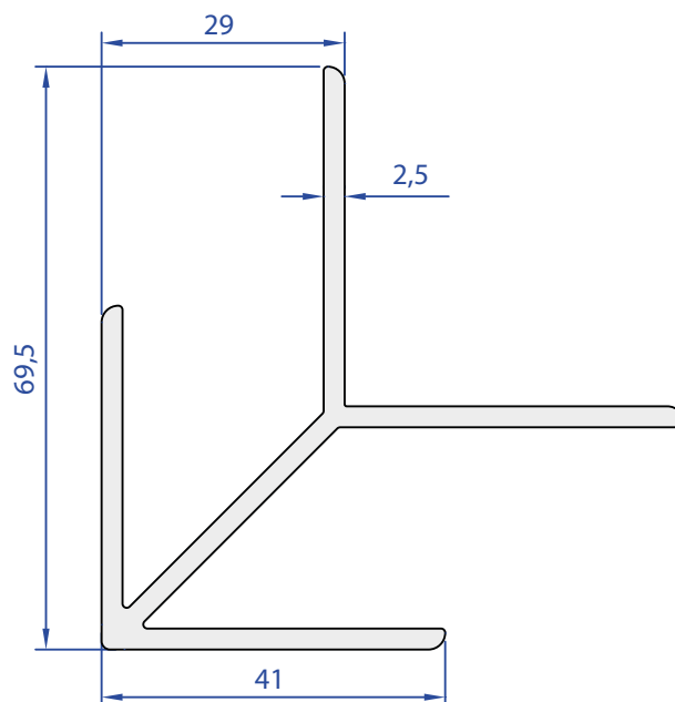
81008-00 1,325 kg/m
