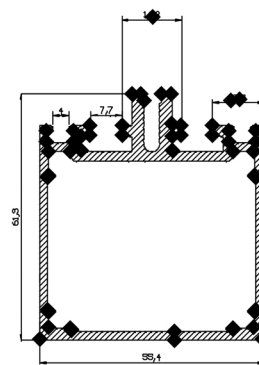
83035-00 1,613 Kg/m
