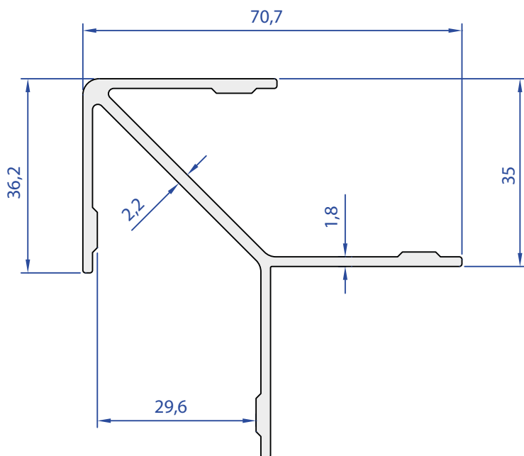
85005-00 1,039 Kg/m
