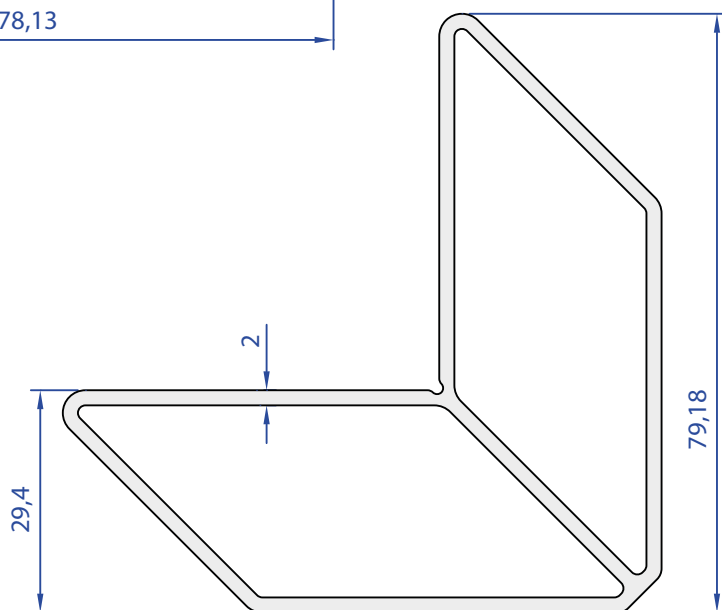
06954-00 1,673 Kg/m
