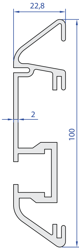
60008-00 1,375 kg/m
