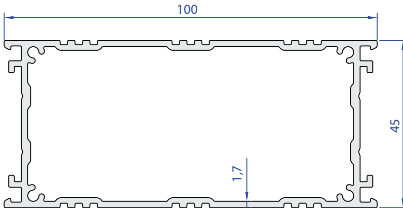
05912-00 1,585 Kg/m
