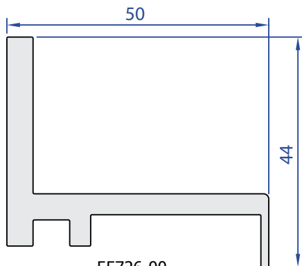
55726-00 1,154 Kg/m
