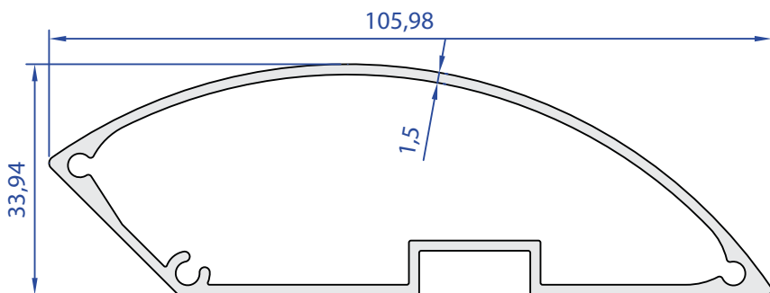
55696-00 1,085 Kg/m
