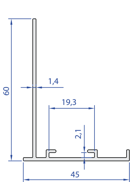
55708-00 0,444 Kg/m
