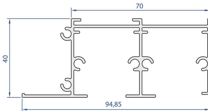
55754-00 1,100 Kg/m
