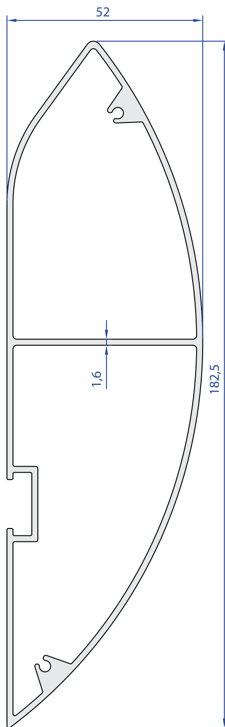
55403-00 2,201 Kg/m
