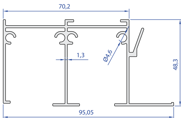
55649-00 1,175 Kg/m
