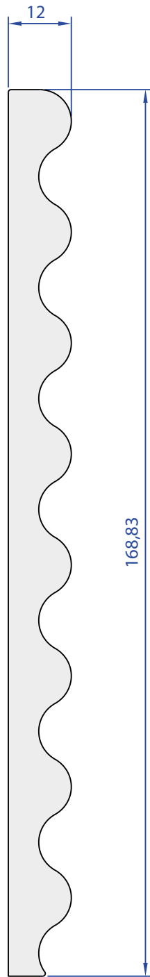
06505-00 4,066 Kg/m
