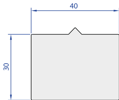
05843-00 3,263 Kg/m
