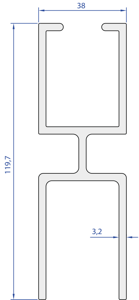
07198-00 2,617 Kg/m
